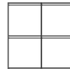
4/D SWINGING WARDROBE PJMN0012 With 4 doors, 2 shelves and 4 hanging rods inch W 90" D 24" H 94" cm L 228,7 P 61,5 H 239,1 Crts 8 kg 366 m 3 0,51
