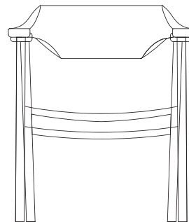
SOHO DINING CHAIR - PEWTER H: 750 W: 640 D: 500
