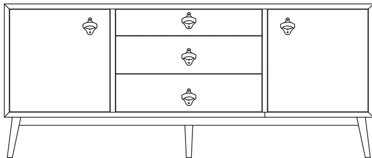
LARGE SIDEBOARD H: 762 W: 1828 D: 482
