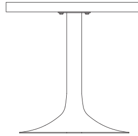
SIDE TABLE - LARGE H: 609 W: 381 D: 635
