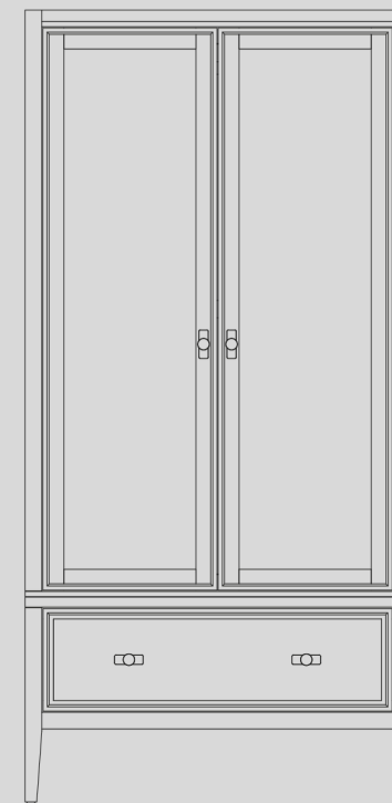
1 DRAWER WARDROBE H: 1900 W: 920 D: 580
