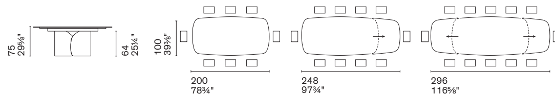
CS4153-S 200 / CS4153-S 200 MTO
